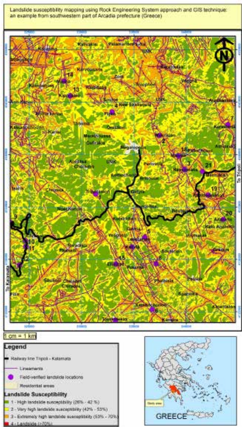
Figure 7: Landslide susceptibility map of Megalopolis area scaled in 1:100,000 (Tavoularis, 2017).
