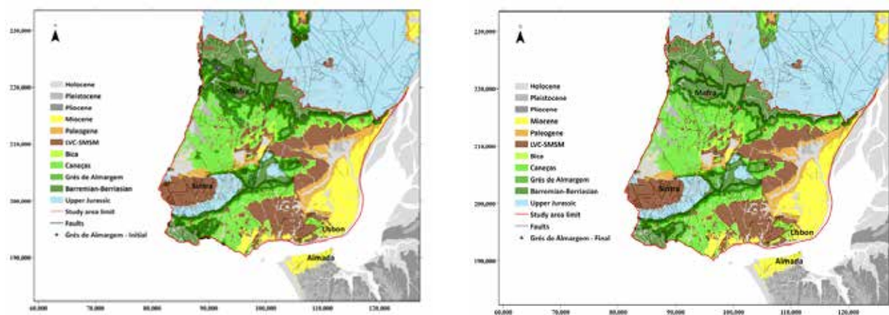
Figure 2: Grés de Almargem points before (left) and after (right) the refinement of boundaries.
