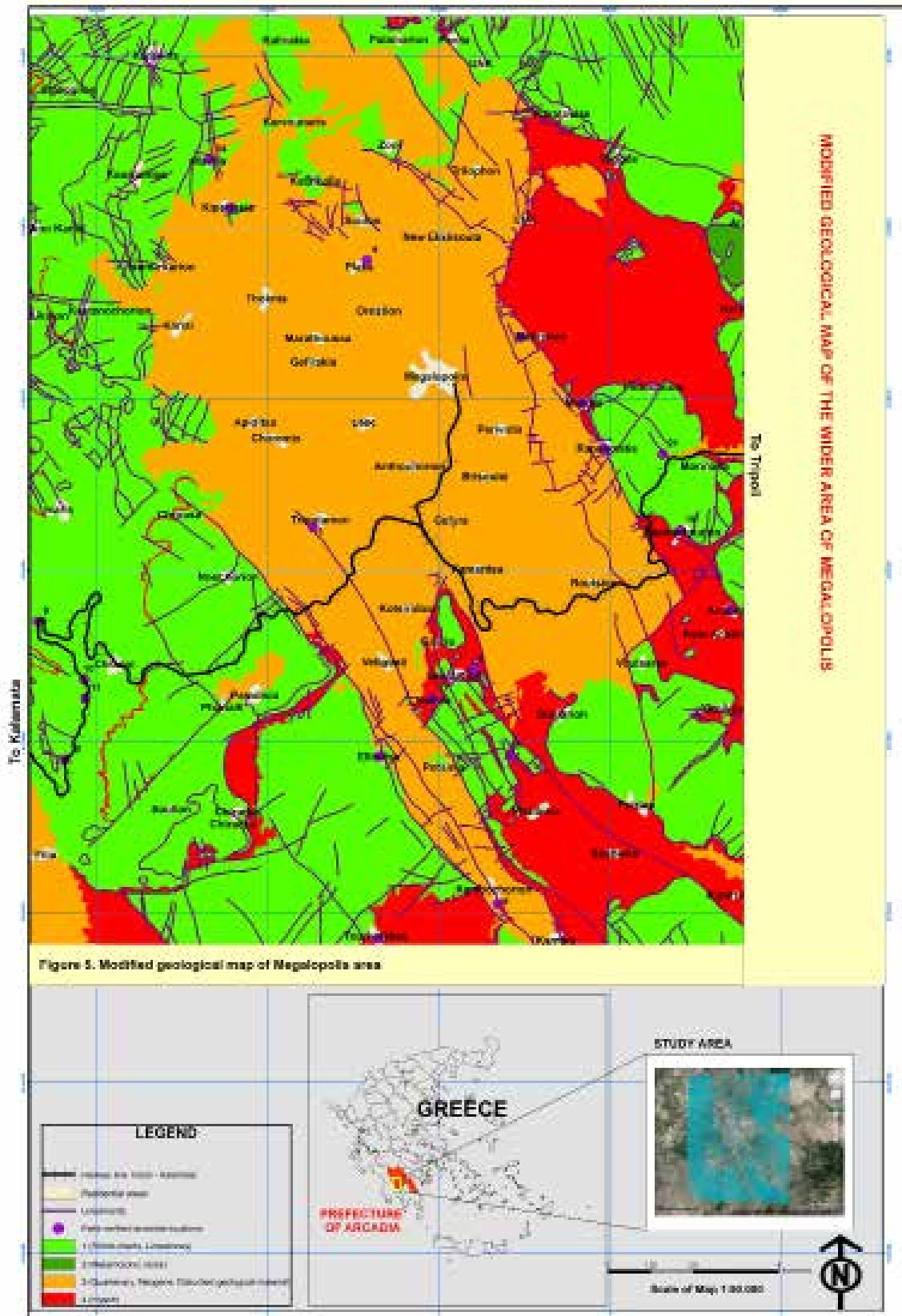
Figure 5: Modified geological map of Megalopolis area, scale 1:100,000 (Tavoularis, 2017).
