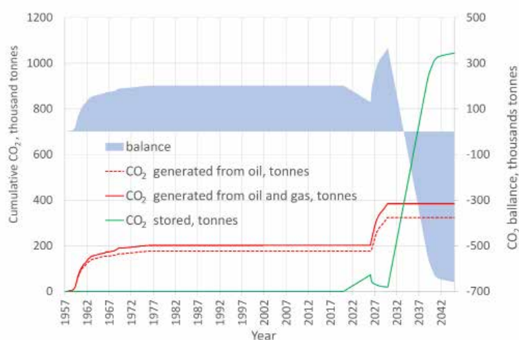
Figure 3: CO 2 balance of one of the initial simulations for the LBr-1 field. On the horizontal (time) axis we can identify the historical phase of conventional oil production, the long relaxation period after site abandonment, and the potential future CO 2 -EOR and CO 2 storage phases.
