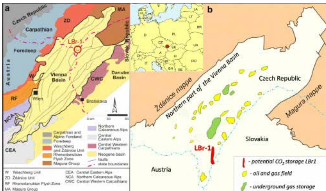
Figure 2: Sketch maps of the whole Vienna Basin (a) and its Northern part (b) with the location of the LBr-1 field (Francu et al., 2017, adapted from Kováč et al., 2008).
